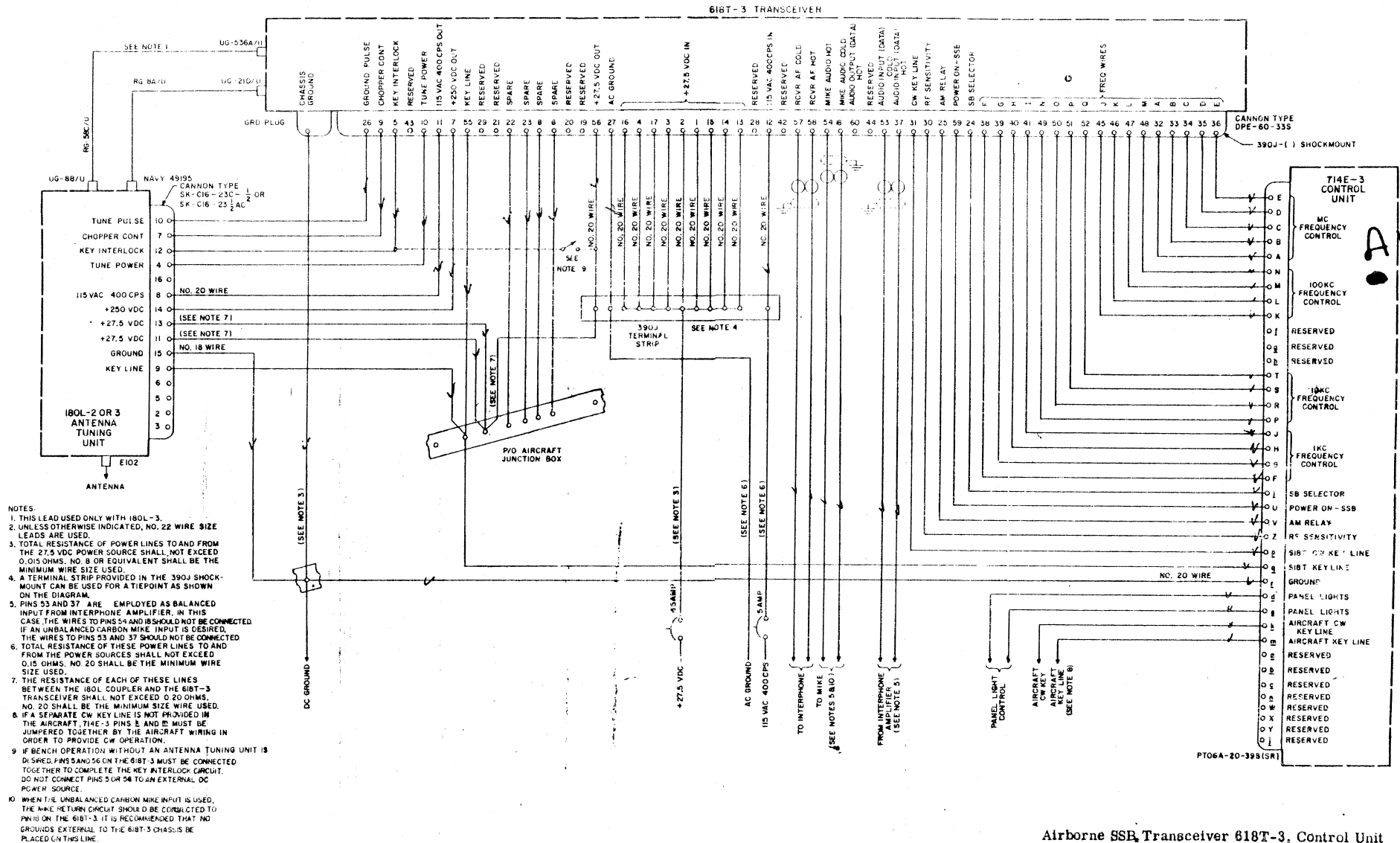
Airborne SSB Transceiver 618T-3, Control Unit 714E-3, and Antenna Tuner 180L-(-), Interconnecting Wiring Diagram Figure 123
